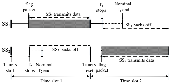
Fig. 2. Example of 2 subsystems competing for the channel in 2 successive time slots. Subsystem 1 (denoted as SS_1 ) has the largest induced error in the first time slot and gets the access to the channel. Subsequently, subsystem 2 (denoted as SS_2 ), that did not communicate in the first time slot, in the second time slot gets to have a larger induced error. Here, m_{2,2} > m_{1,2} and thus SS_2 gets access to the channel.
