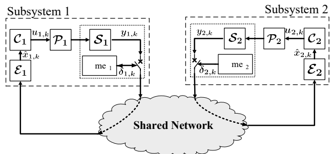
Fig. 1. Example of the NCS layout where two subsystems compete to transmit their local measurements through the limited capacity shared network. \mathcal{P}_i represents the plant of subsystem i \in \{1, 2\} , \mathcal{S}_i its sensor, \mathcal{E}_i its estimator, and \mathcal{C}_i its controller. Note that the timer is embedded in the sensor.
