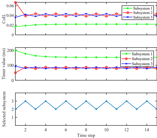
Fig. 3. Resource allocation with TBCoIL for a simple case of two unstable subsystems and a stable one sharing a single channel. Since the CoIL for unstable subsystems is always higher, their timers expire faster and the channel is dedicated to them.
