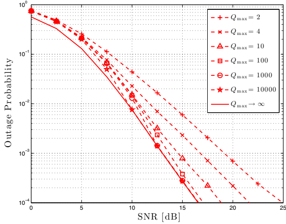
Fig. 3. Outage probability of the proposed BA-PARS scheme for varying the maximum buffer size Q_{\max} when C_0 = 1 BPCU and K = 3 . The convergence occurs at lower buffer sizes at high SNR than at low SNR.
