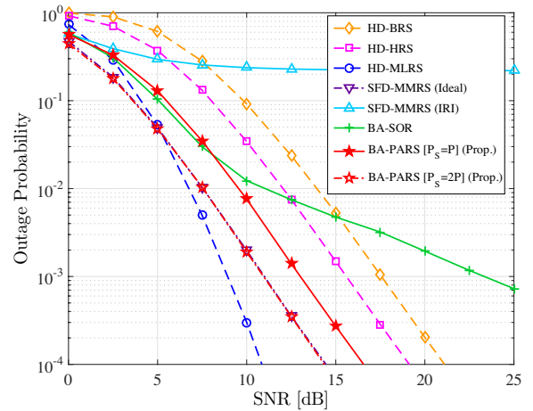
Fig. 2. Outage probability for C_0 = 1 BPCU, K = 3 , and Q_{\max} \rightarrow \infty . For the proposed BA-PARS scheme, we additionally consider double power at the source (denoted by ‘[2P]’) to show the case of a powerful source node.
