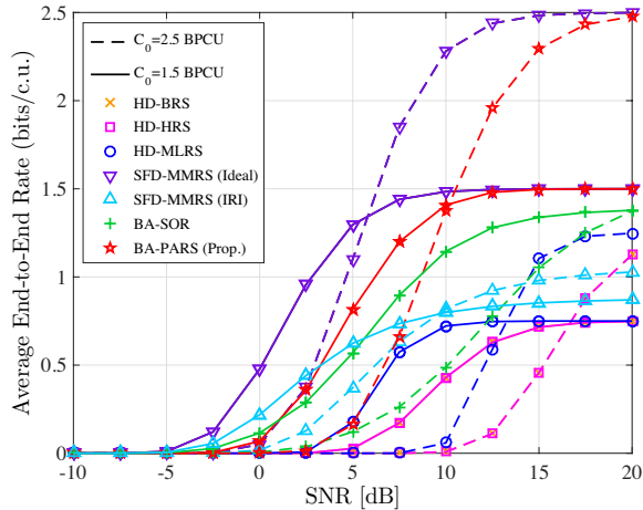
Fig. 4. Average end-to-end rate with three different fixed data rates ( C_0 = 1.5 and C_0 = 2.5 BPCU) when K = 3 and Q_{\max} = 10 .
